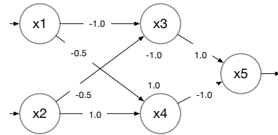
Fig. 1: A DNN with 2 inputs, 2 hidden neurons, and 1 output.
