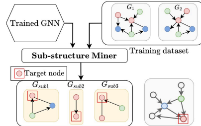
Fig. 4: Influential substructures and graph isomorphism.
