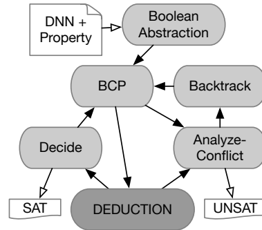
Fig. 2: NeuralSAT Overview.
